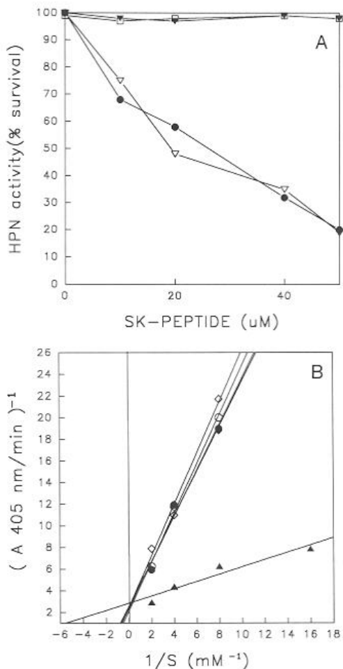
Fig. 3. Dose-dependent inhibition of plasmin activity by HPG binding peptides. A: Amidolytic activity of fixed amounts of HPN (0.4 \mu\text{M} ) was measured in the presence of varying concentrations of synthetic SK peptides (0–50 \mu\text{M} ), and the percent survival of HPN activity was then quantitated. Different reactions contained either SK234–253 (open triangles), SK254–273 (closed triangles), or SK274–293 (closed circles). B: Effect of SK and SK peptides on the kinetic parameters of HPN for amidolysis of G-P-L-pNA. SK (closed circles) (0.12 \mu\text{M} ), SK143–293 (open circles) (0.5 \mu\text{M} ), and SK peptides (80 \mu\text{M} ) viz., SK234–253 (open squares) and SK274–293 (closed inverted triangles), were incubated with HPN and the amidolytic activity in the presence of varying concentrations of G-P-L-pNA (0.06–0.5 mM) were then estimated. Lineweaver–Burke plots of the data are shown. HPN alone (closed triangles) was taken as control.
