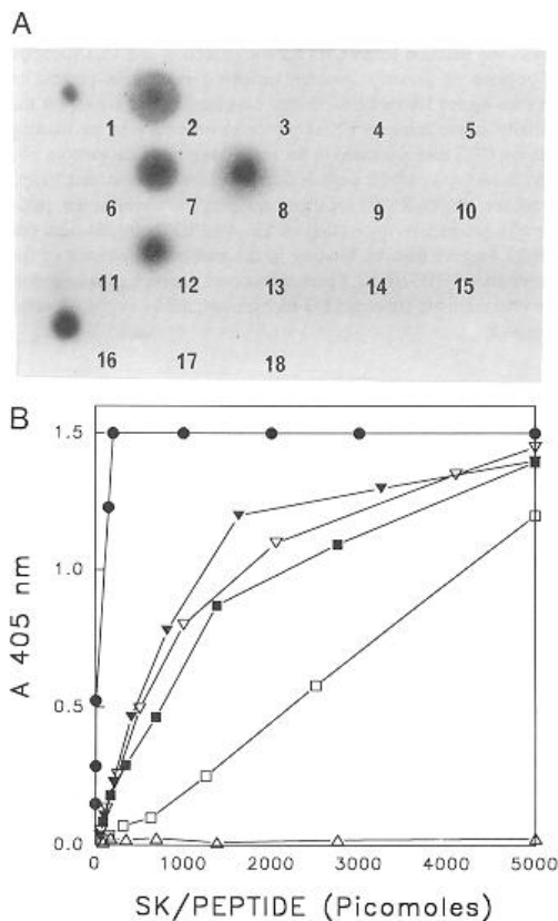
Fig. 1. Plasminogen binding analyses of synthetic peptides by dot blot and ELISA. A: Dot blots showing binding of radiolabeled HPG to SK peptides. Positions marked 1 and 2 correspond to SK ( 1 \mu\text{g} ) and SK143–293 ( 5 \mu\text{g} ), respectively, whereas 7, 8, 12, and 16 represent SK234–253, SK254–273, SK274–293, and SK263–282, respectively. B: Quantitative ELISA for HPG binding. Plots show binding of either SK (closed circles) or SK peptides viz., SK234–253 (open inverted triangles), SK254–273 (closed triangles), SK274–293 (closed squares), and SK263–282 (open squares), with HPG. Control reaction where SK or SK-peptides were omitted is depicted with open triangles.
